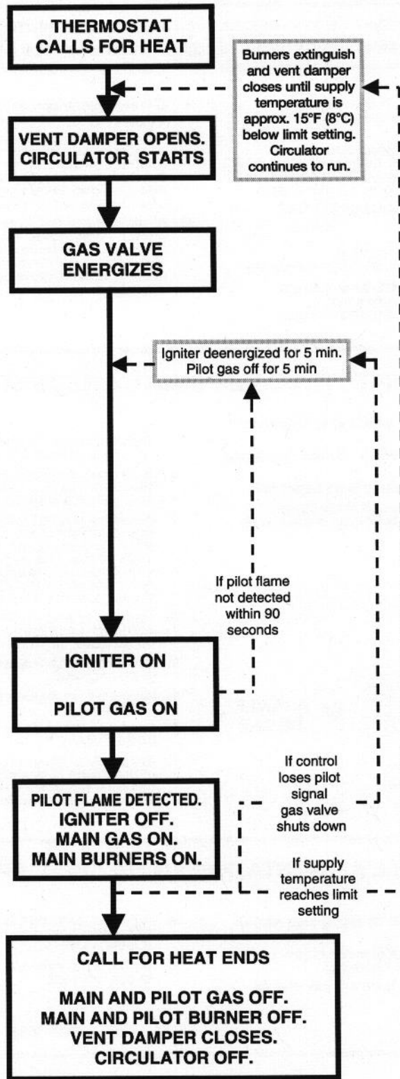
Figure 4: Intermittent Ignition Sequence of Operation
