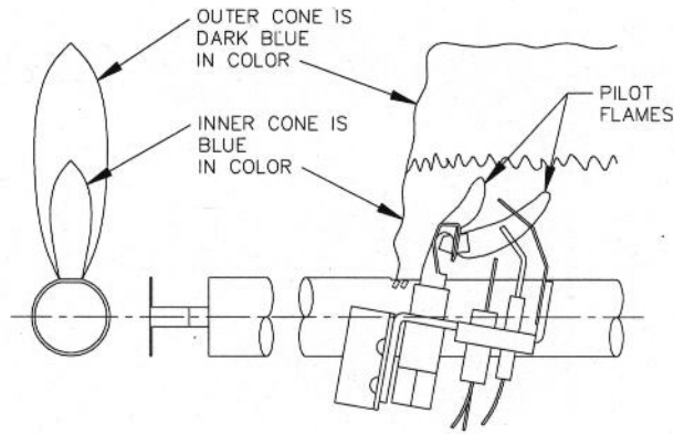
Figure 5: Intermittent Ignition Pilot Configuration and Flames
